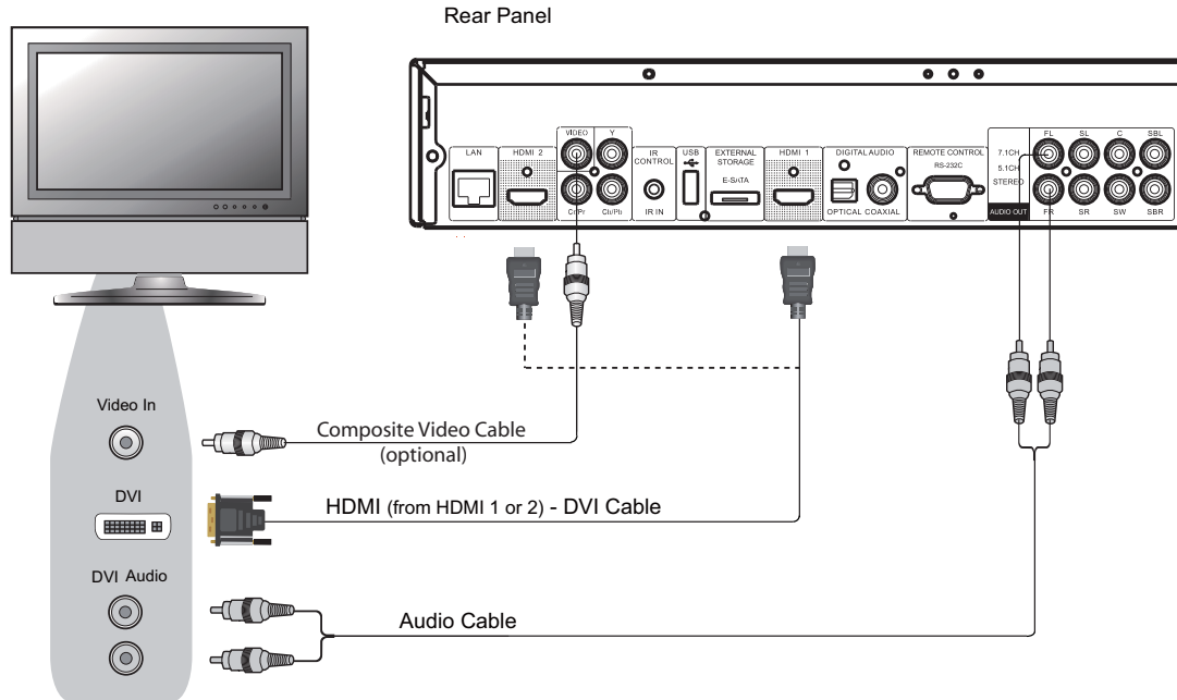
Method 2 – DVI Connection to TV
